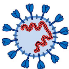
SARS COV 2
